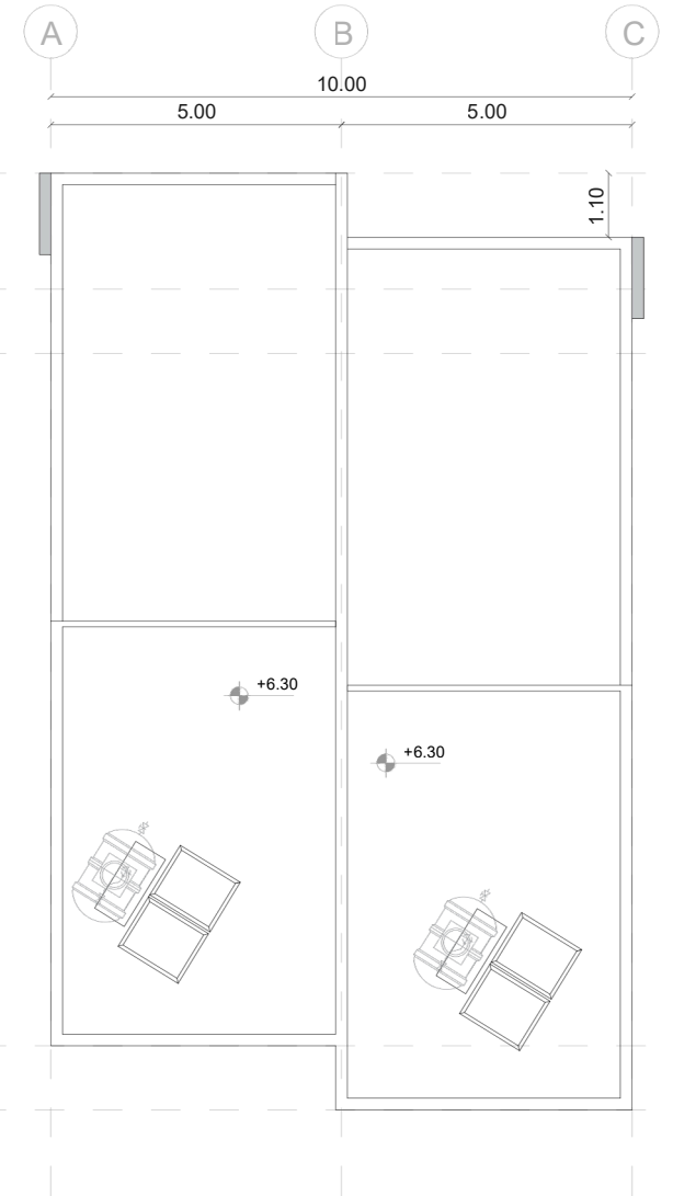
ROOF PLAN
